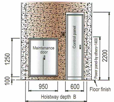
Opening for Control panel & Maintenance door
