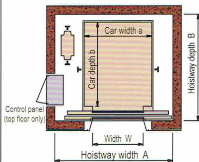
T1 type Hoistway plan
