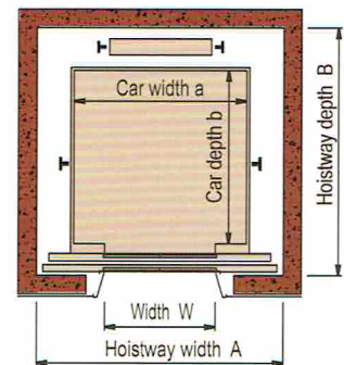
Hoistway plan
