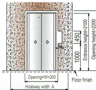
Entrance plan
