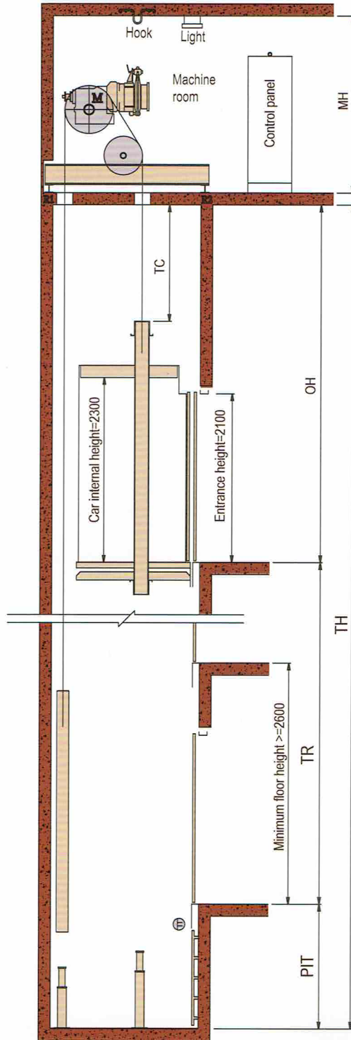
Hoistway section
