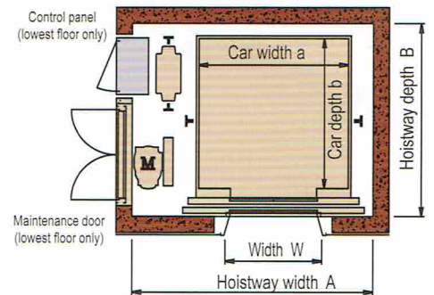
RL-c Hoistway plan (Machine at right side or left side)
