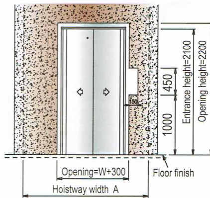
Entrance plan
