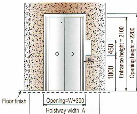
Entrance plan
