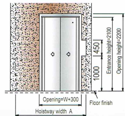
Entrance plan
