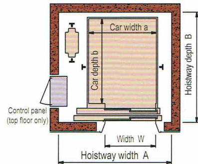
T3 type Hoistway plan
