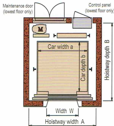
RL-b Hoistway plan (Machine at rear side)
