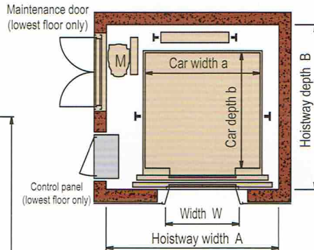
RL-a Hoistway plan (Machine at right side or left side)
